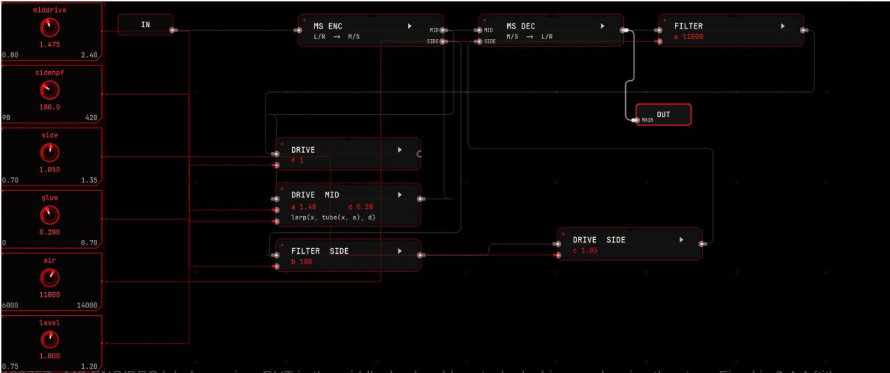
183757 - MS ENC/DEC labels on pins, OUT in the middle, knob cables stacked, chips overlapping the story. Fixed in 0.4.4 (title row, no overlap, OUT to the right, curved knobs).
